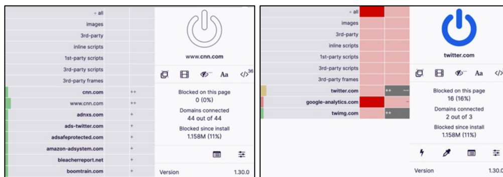
Figure 9.03: Fully and partially enabled scripts with uBlock Origin.
