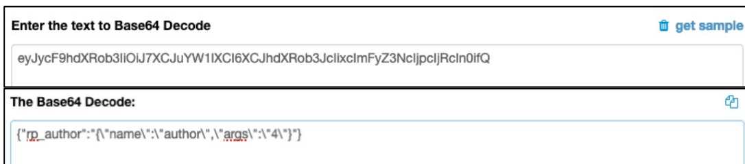
Figure 18.06: Decoding text to Base64 on https://codebeautify.org/base64-decode .
