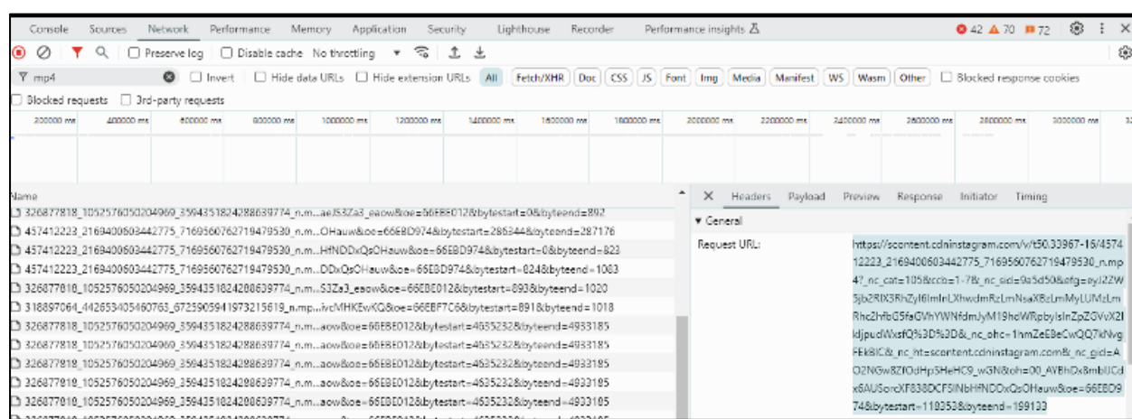
Figure 20.06: The "Inspector" utility within Firefox identifying an Instagram video MP4 file.
